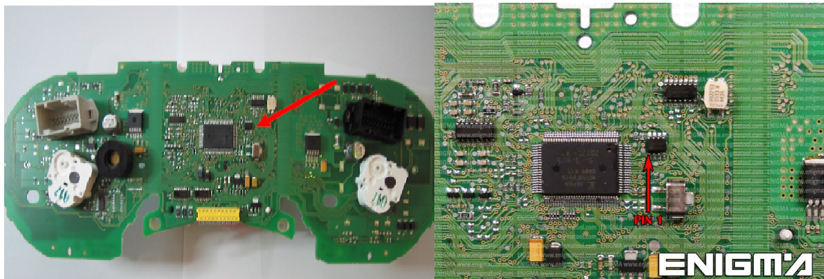
PHOTO 1: Connect cable C4 to the Eeprom memory according to the picture above.
