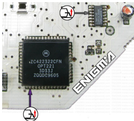
PHOTO 1: Solder cable and lift PINS like shown on the photo above.
