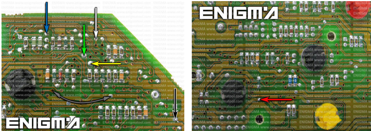
PHOTO 2: Solder cables according to the colors like shown on the photos above.
