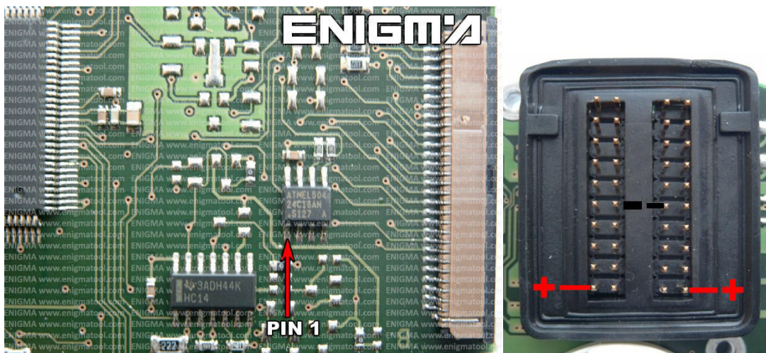
PHOTO 1: Connect cable C4 to the Eeprom memory according to the picture above. Second picture shows us power lead connection.
