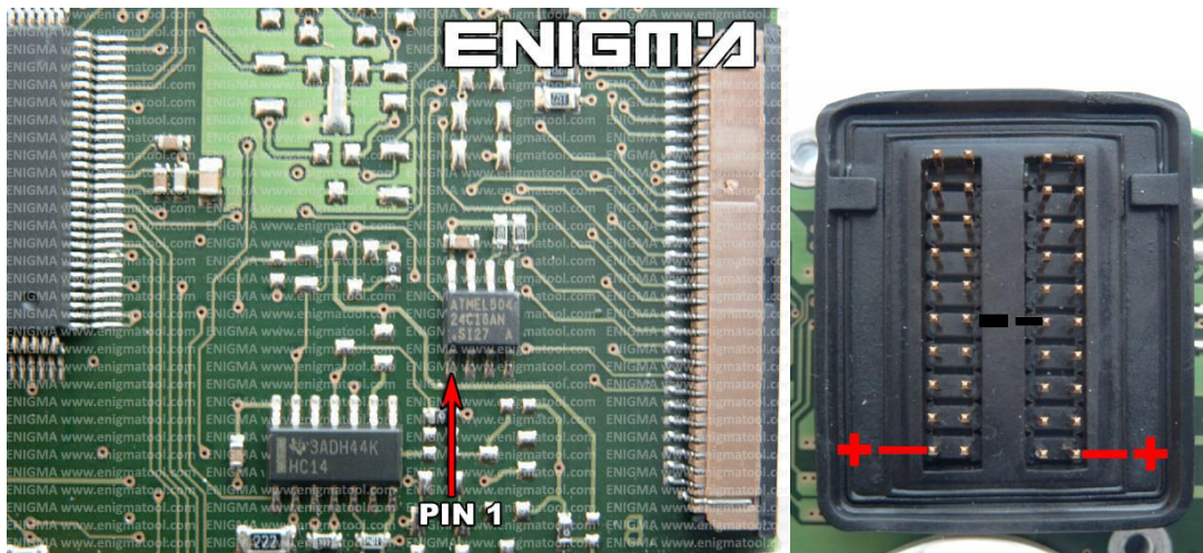
PHOTO 1: Connect cable C4 to the Eeprom memory according to the picture above. Second picture shows us power lead connection.
