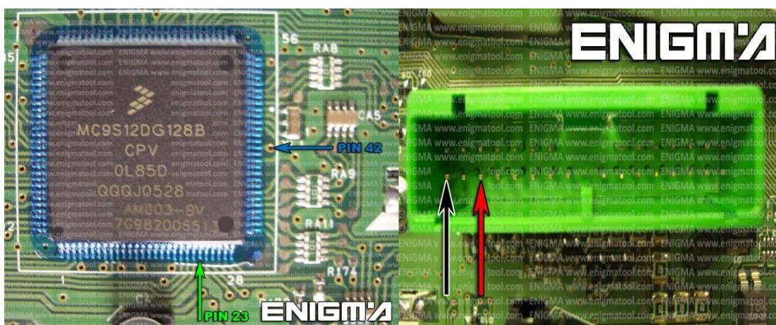
PHOTO 1: Solder cables according to the colors shown on the pictures above.
