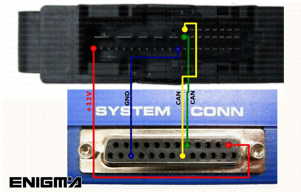
PHOTO 2: Make connection as shown on the photo above.
