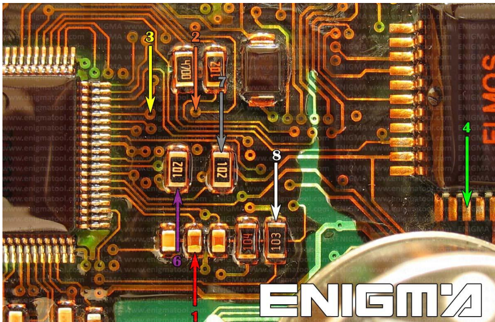
PHOTO 1: Solder C7 cables according to the picture above.
