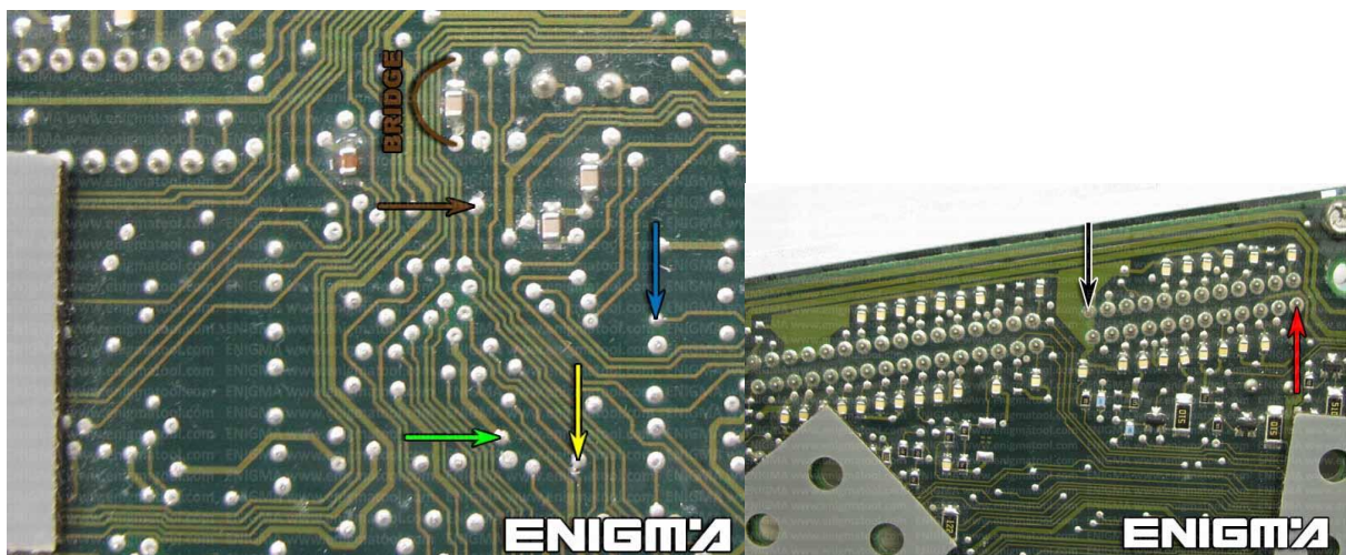
PHOTO 1: Solder C11 cables according to the colors like shown on the photos above.
