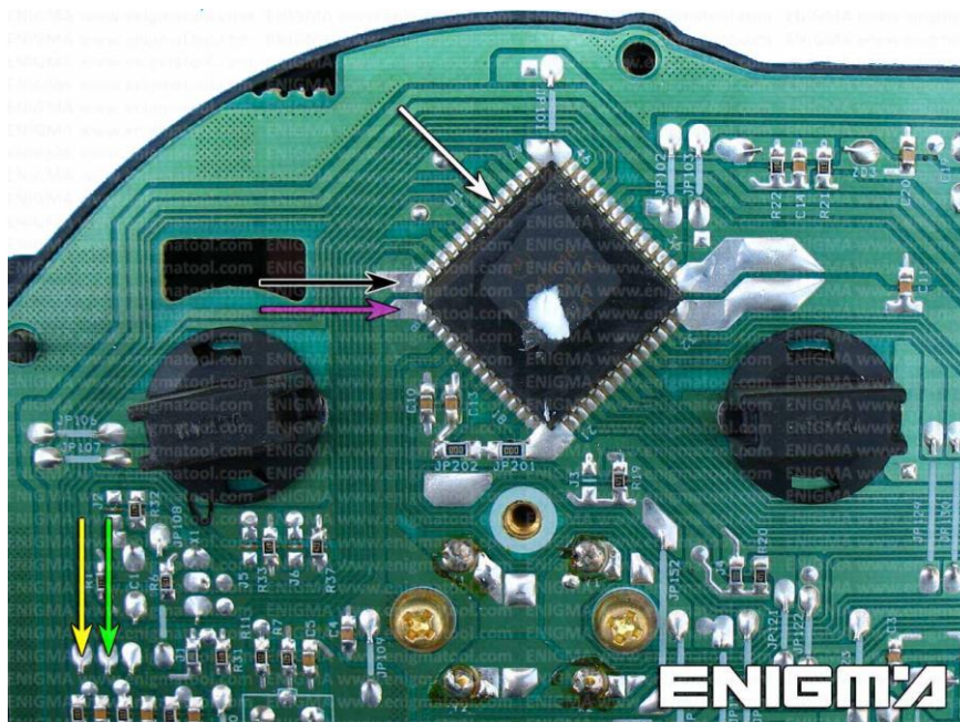
PHOTO 1: Solder C11 cables according to the colors like shown on the photos above.
