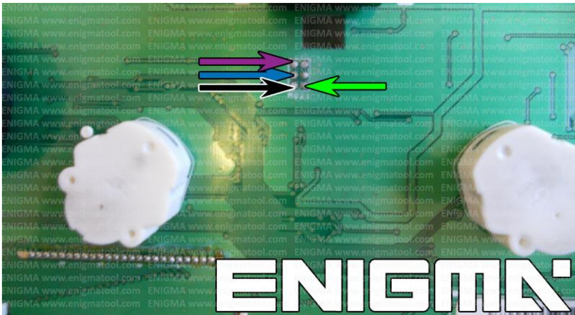
PHOTO 1: Solder C12 cables according to the colors like shown on the photos above.
