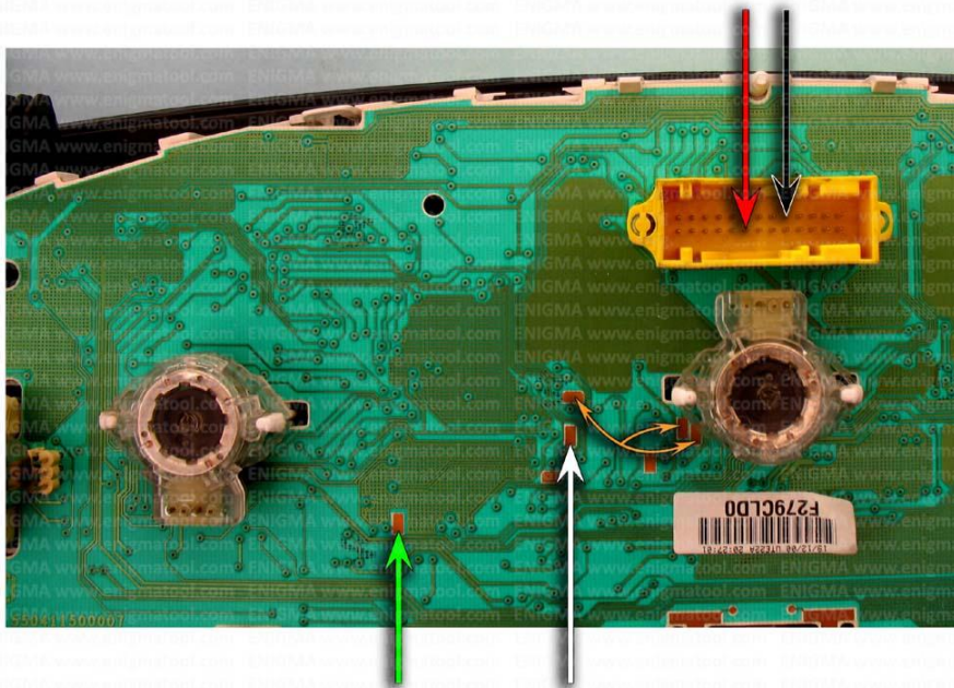
PHOTO 1: Solder C12 cables according to the picture above.
