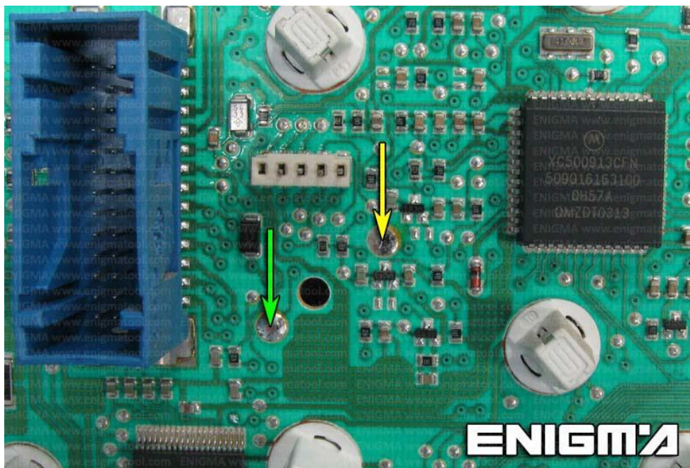
PHOTO 1: Solder C11 cables according to the picture above.
