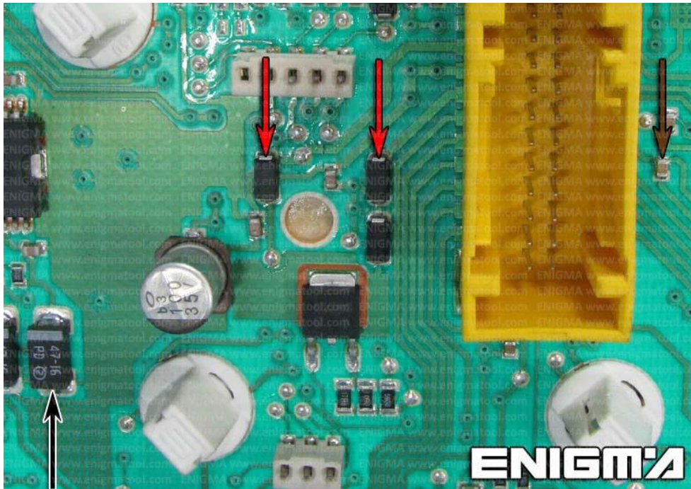
PHOTO 2: Solder C11 cables according to the picture above.
