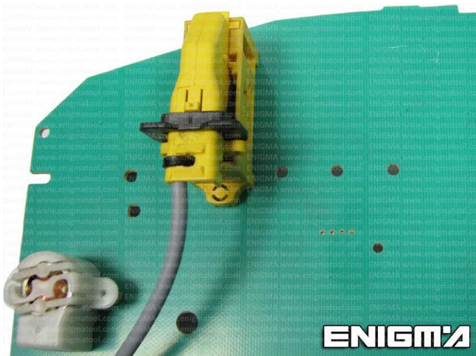
PHOTO 1: Connect cable C20 like shown on the photo above.
