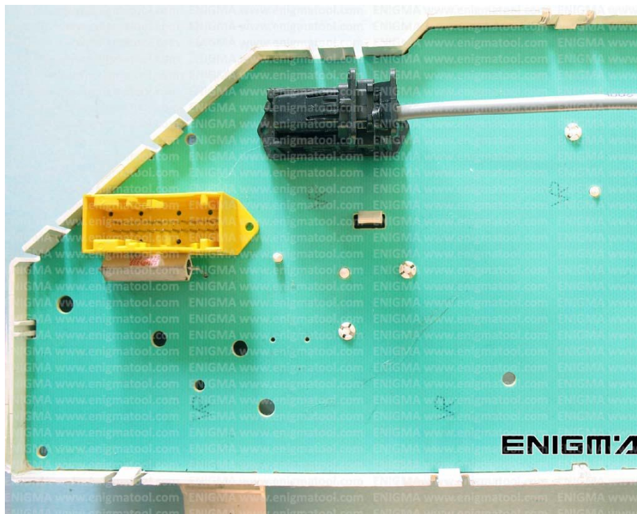
PHOTO 1: Connect cable C21 like shown on the photo above.
