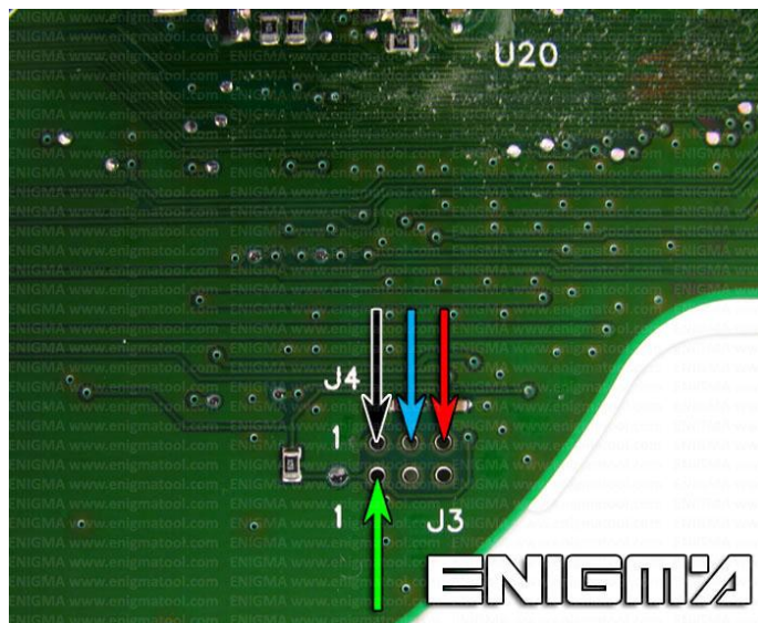
PHOTO 1: Solder C45 cables as shown on the photo above.
