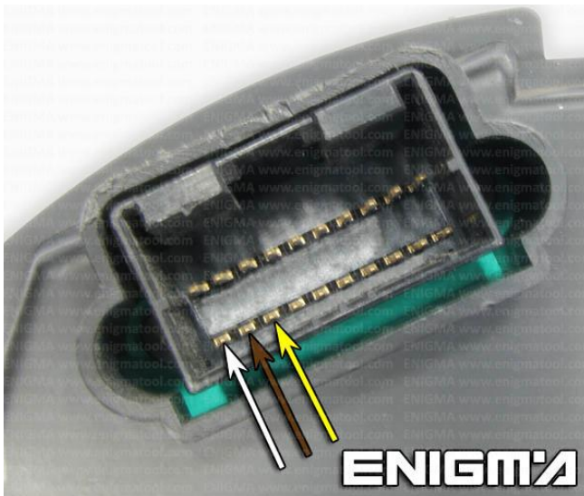
PHOTO 1: Connect cable C15 to the points as show on the picture above.
