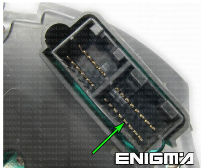
PHOTO 1: Connect cable C15 to the points as show on the picture above.
