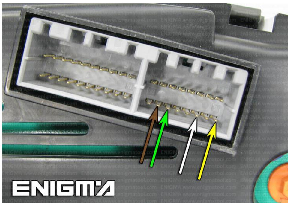
PHOTO 1: Connect cable C15 to the points as show on the picture above.
