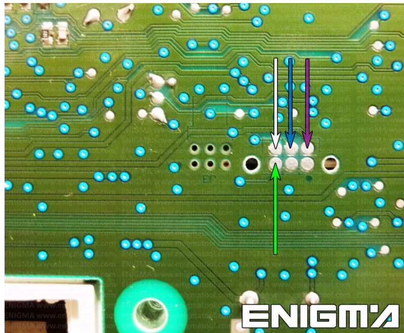
PHOTO 1: Solder C12 cables according to the colors like shown on the photos above.
