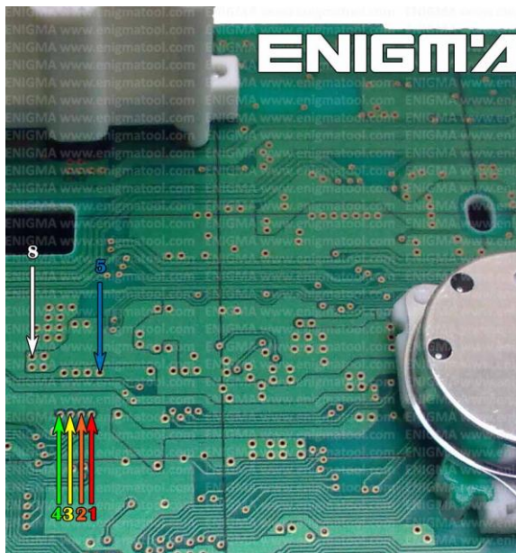
PHOTO 1: Solder cable C7 to points according to the picture above.
