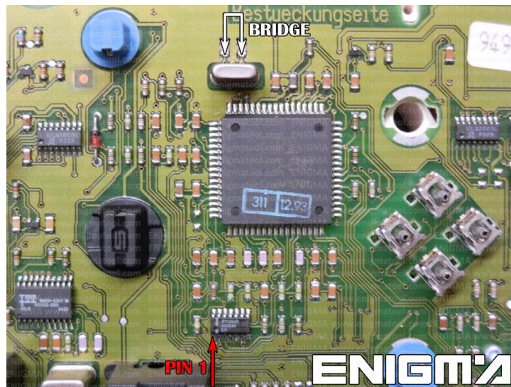
PHOTO 1: Connect cable C6 to the EEPROM memory according to the picture above.
