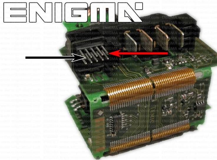
PHOTO 2: Solder C12 cables according to the colors like shown on the photo above.
