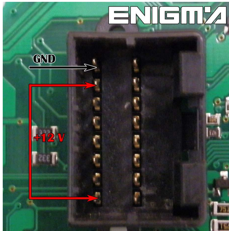
PHOTO 2: Power lead connection.
