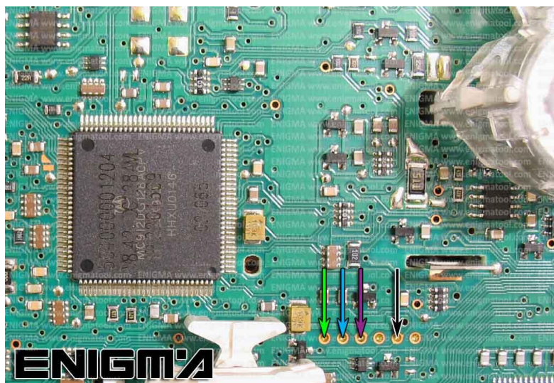
PHOTO 1: Solder cables according to the colors like shown on the photo above.
