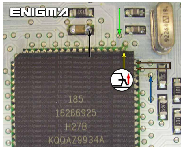
PHOTO 1: Solder C11 cables according to the colors like shown on the photo above.
