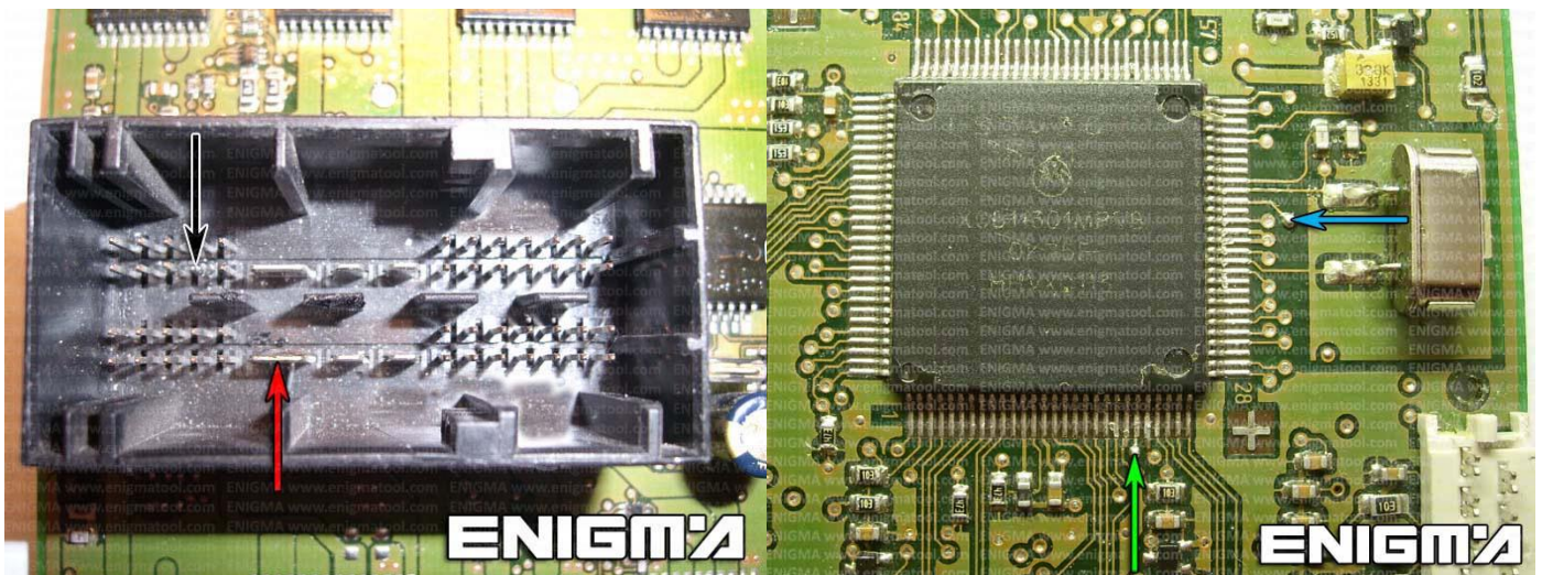
PHOTO 1: Solder cable C12 according to the pictures above.
