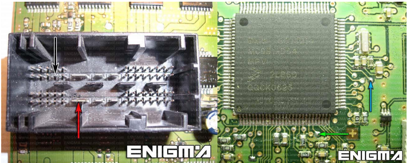
PHOTO 1: Solder cable C12 according to the pictures above.
