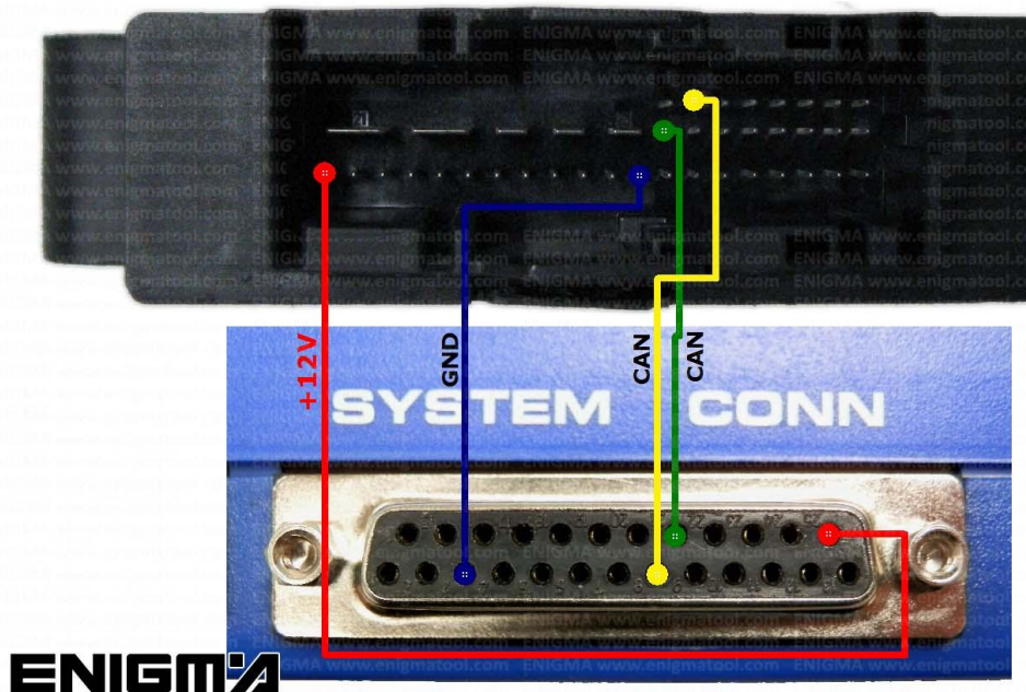
PHOTO 2: Make connection as shown on the photo above.
