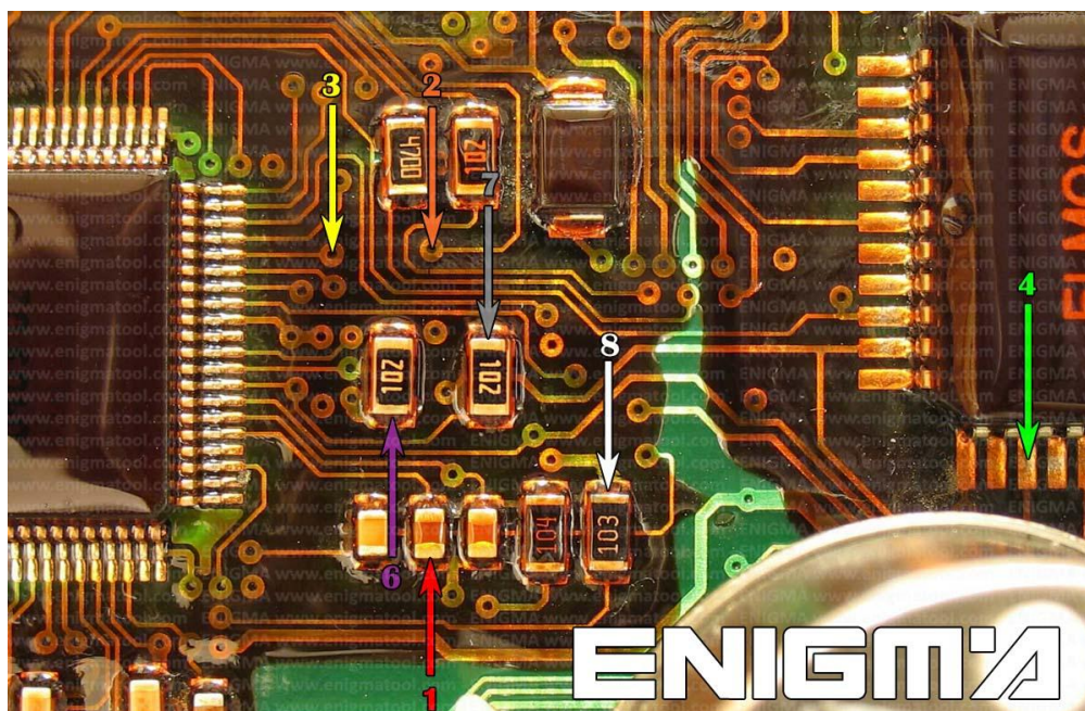
PHOTO 1: Solder C7 cables according to the picture above.
