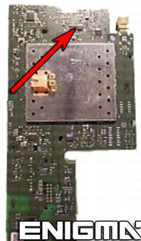
PHOTO 1: Connect cable C4 to the EEPROM memory according to the picture above.
