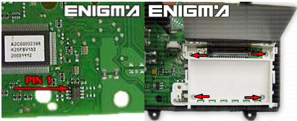
PHOTO 1: Connect cable C4 to the EEPROM memory on the other side of the board after disarming 4 screws according to the picture above.
