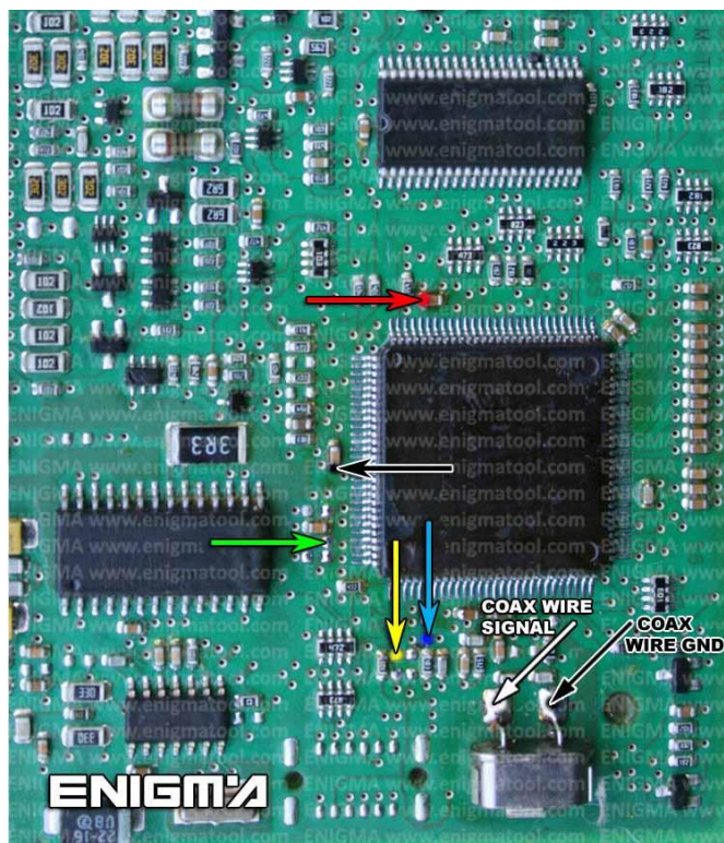
PHOTO 2: Solder C45 cables as shown on the photo above.
