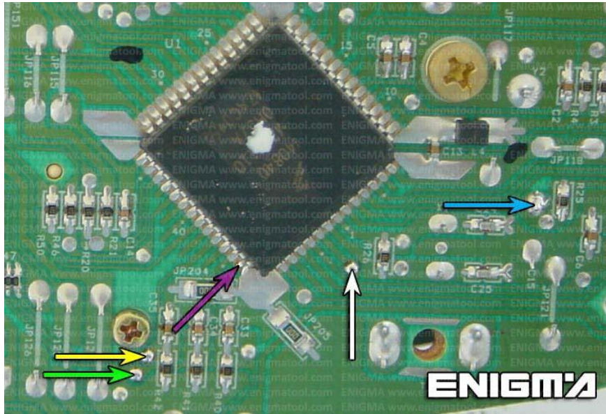
PHOTO 2: Solder C11 cables according to the colors like shown on the photos above.
