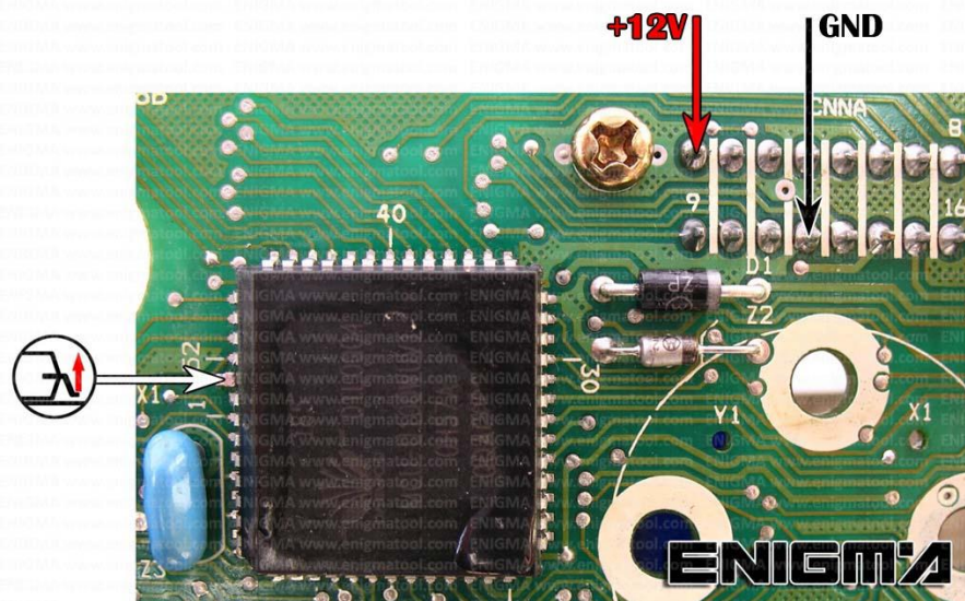
PHOTO 1: Solder C11 cables according to the colors like shown on the photo above.
