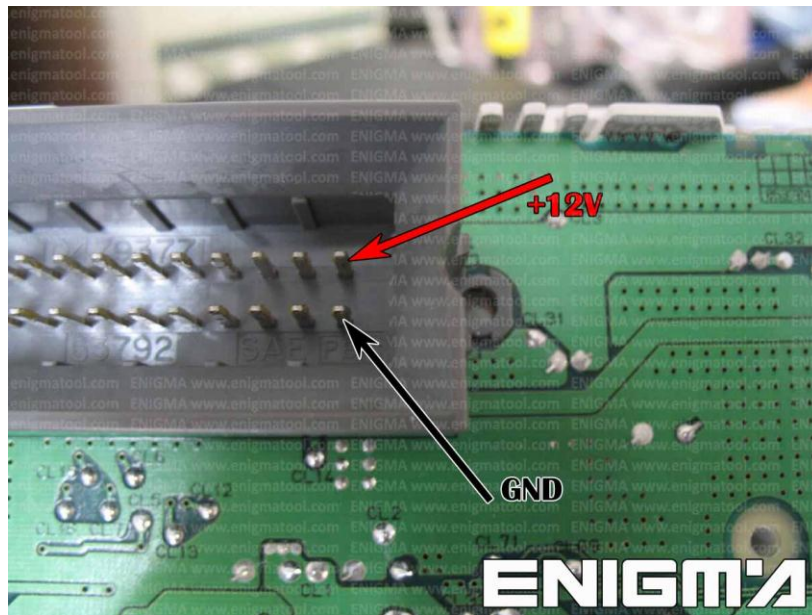
PHOTO 2: Solder C12 cables according to the colors like shown on the photos above.
