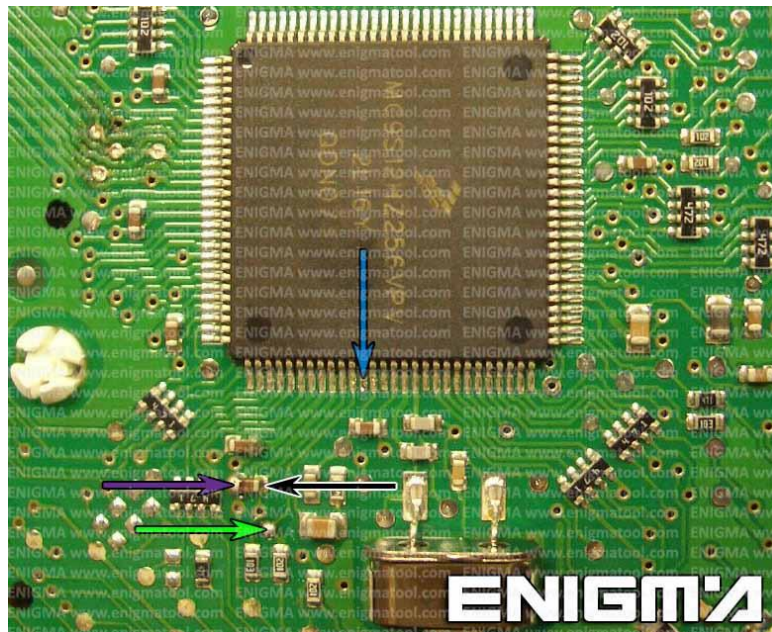
PHOTO 1: Solder C12 cables according to the colors like shown on the photo above.
