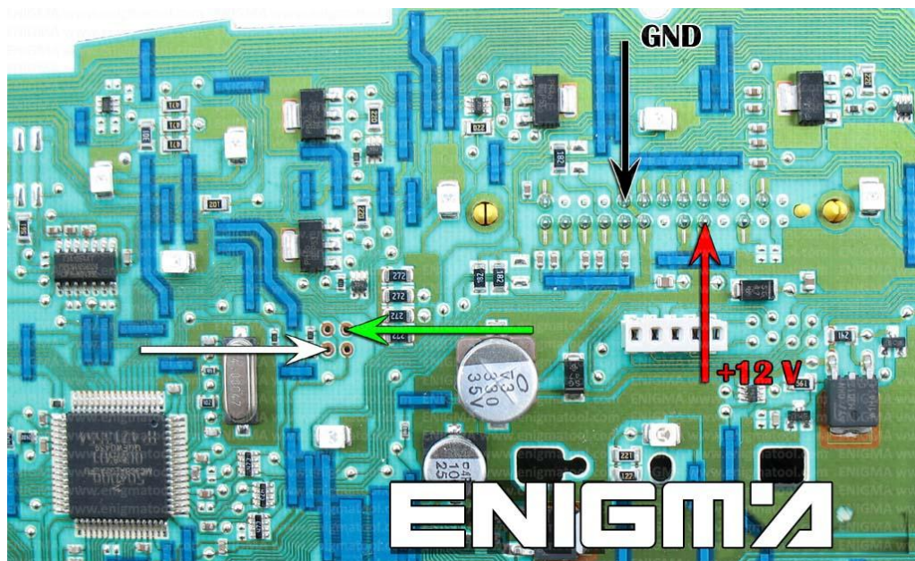
PHOTO 1: Solder C12 cables according to the picture above.
