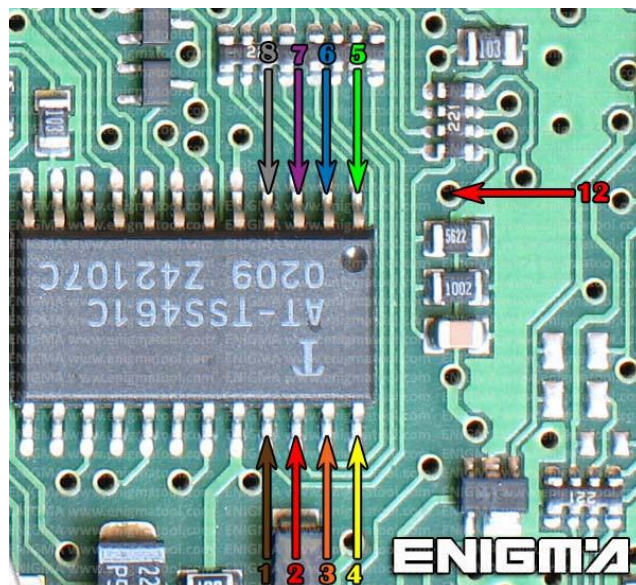
PHOTO 1: Solder C13 cables according to the colors like shown on the photos above.
