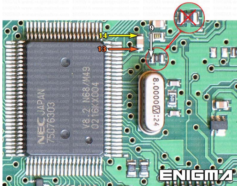
PHOTO 3: Solder C13 cables according to the colors like shown on the photos above. Remember to dismount component shown on photo above and to put it back when the job is done.
