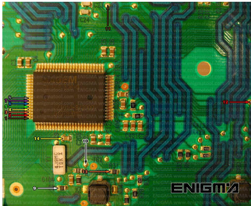
PHOTO 1: Solder C13 cables according to the colors like shown on the photos above.
