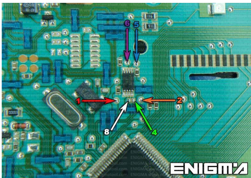
PHOTO 1: Solder cable C7 to points according to the picture above.
