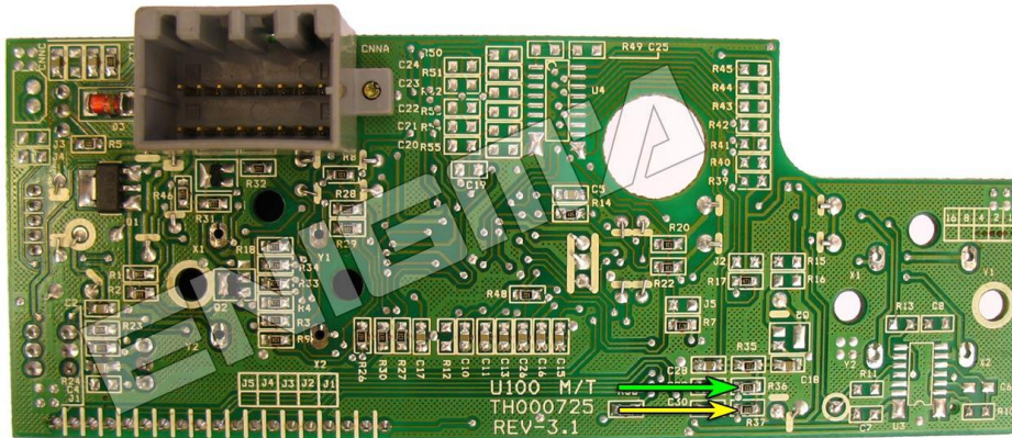
PHOTO 2: Solder C11 cables according to the colors like shown on the photo above.
