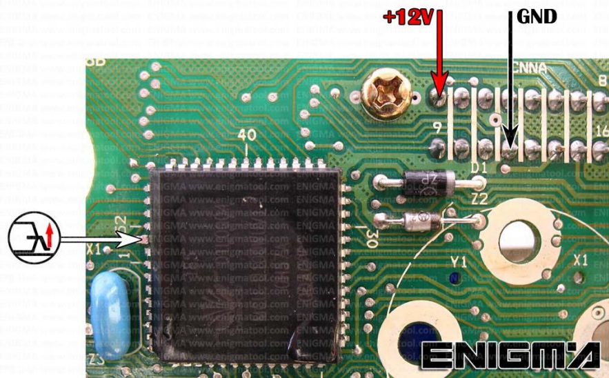
PHOTO 1: Solder C11 cables according to the colors like shown on the photo above.
