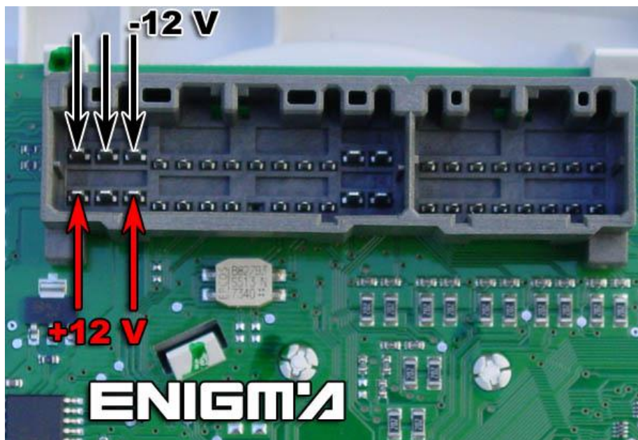
PHOTO 2: Power lead connection.
