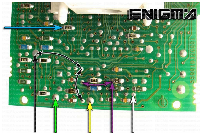
PHOTO 1: Solder cables according to the colors like shown on the photos above.
