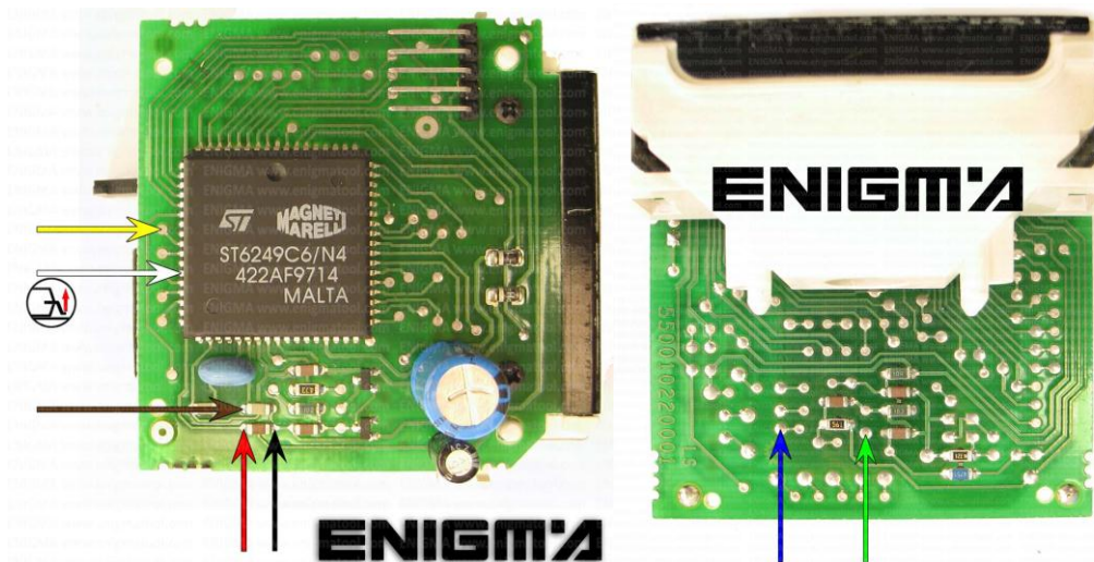
PHOTO 1: Solder C8 cables according to the colors like shown on the photos above.
