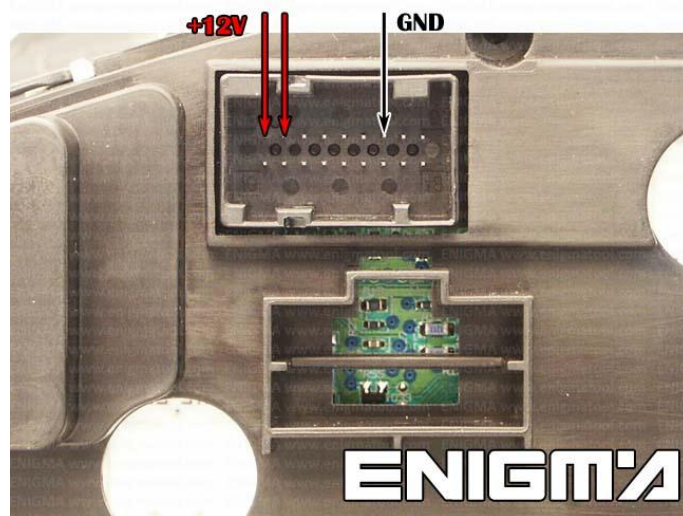
PHOTO 2: Power lead connection.
