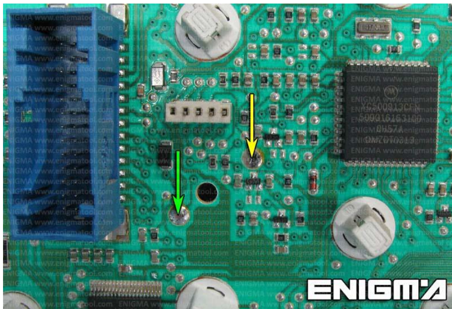
PHOTO 1: Solder C11 cables like shown on the photo above.
