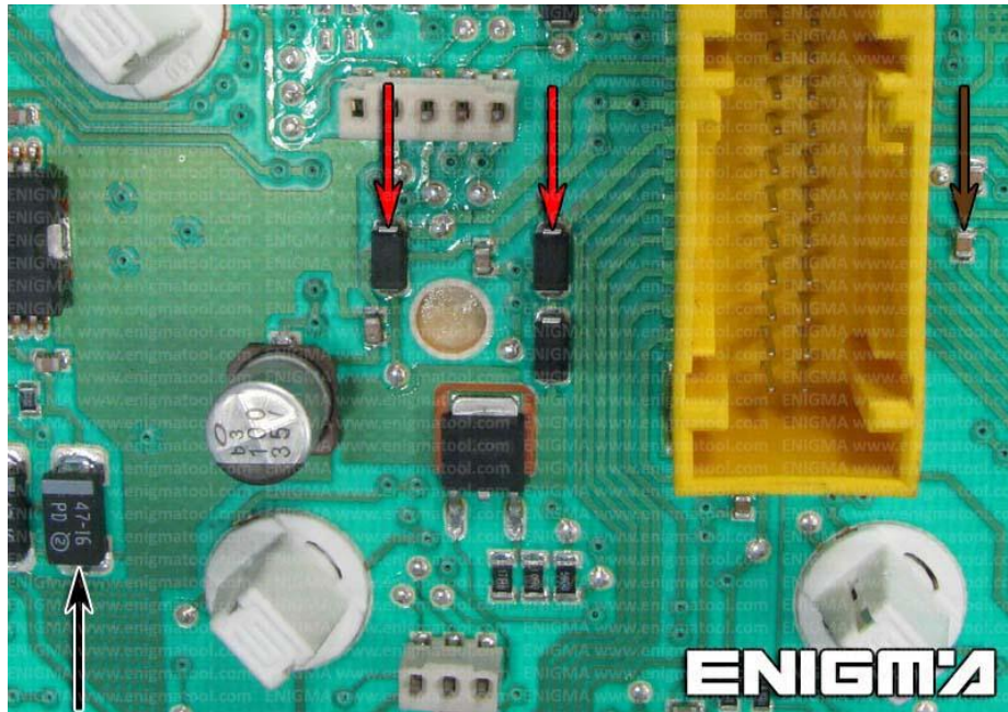
PHOTO 2: Solder C11 cables like shown on the photo above.
