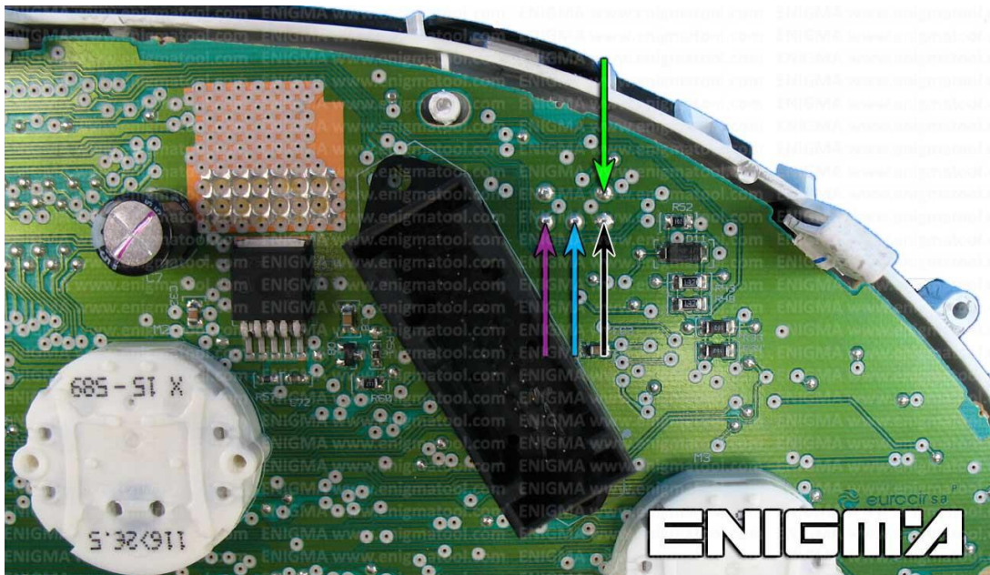
PHOTO 1: Solder C12 cables according to the colors like shown on the photos above.
