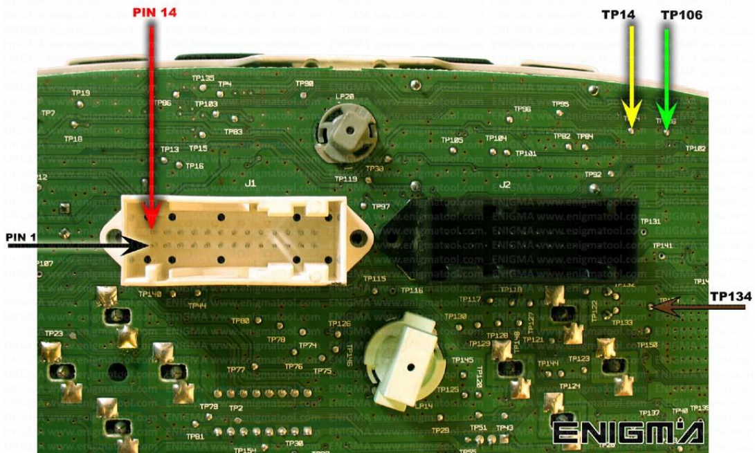
PHOTO 1: Solder C11 cables like shown on the photo above.
