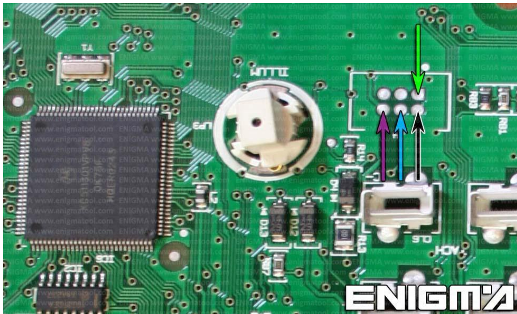
PHOTO 1: Solder C12 cables according to the colors like shown on the photos above.
