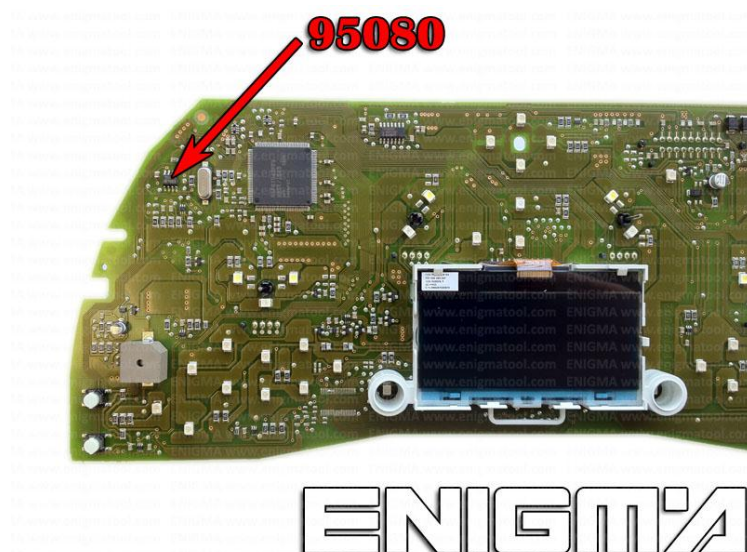
PHOTO 1: Locate the EEPROM memory as shown on the picture above.
