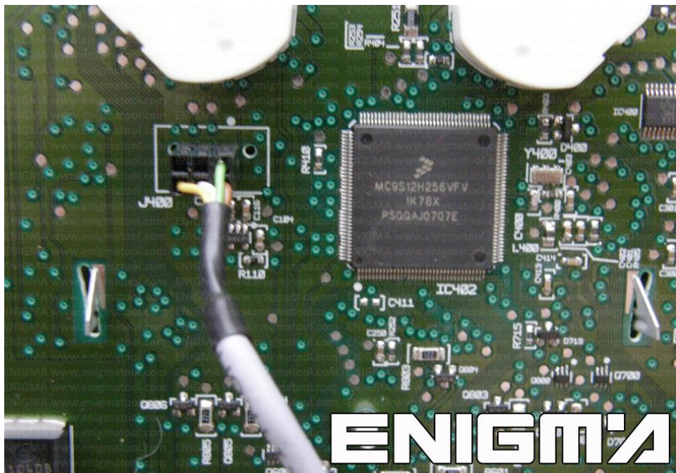
PHOTO 1: Connect C43 cable according to the picture above.
